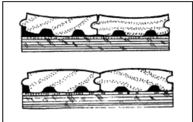
Cupping and crowning action of wet flooring strips provides subsurface air cavities and allows greater air flow.
