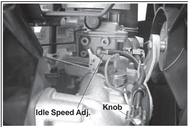
Figure 25. Carburetor and Idle Speed Adjustment.
