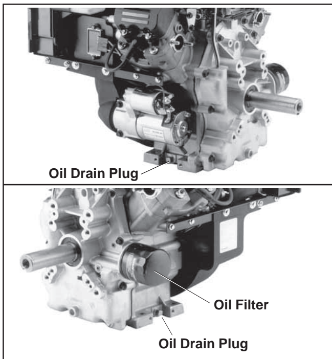
Figure 8. Oil Drain Plugs and Oil Filter.
