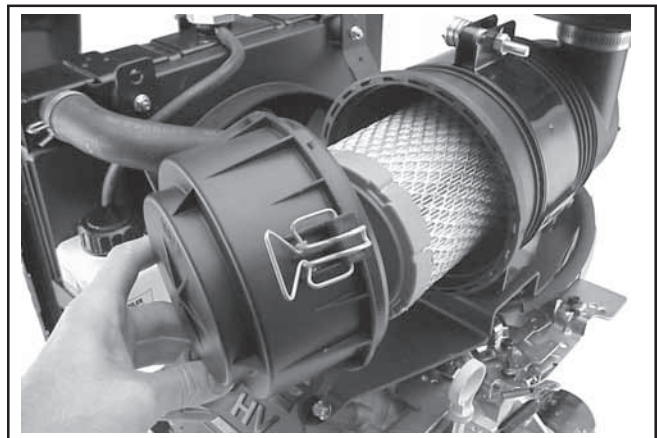
Figure 15. Removing End Cap.
