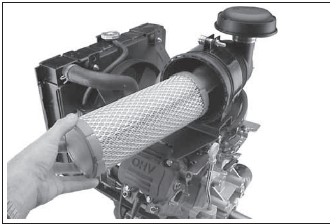
Figure 16. Removing Air Cleaner Element.
