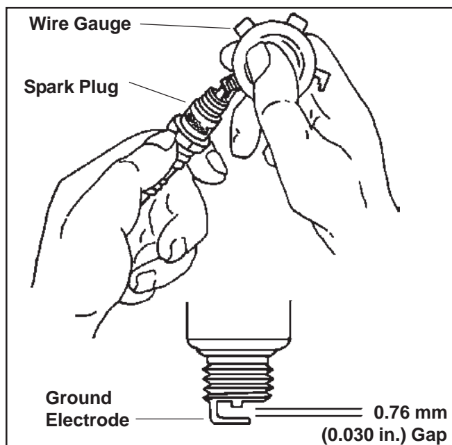
Figure 23. Servicing Spark Plug.
