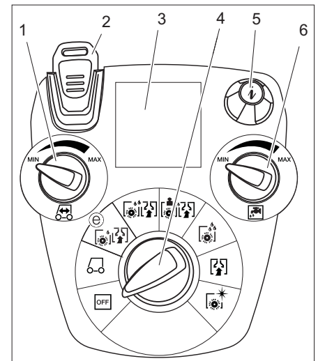
Operator console
