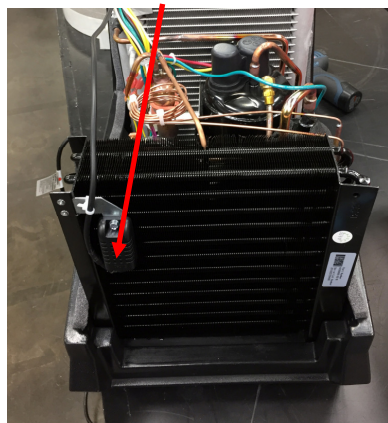
4036924 Control Board
