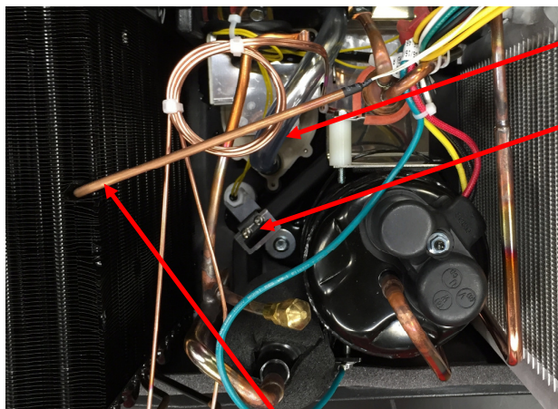
4034716-03 Evap Thermistor
