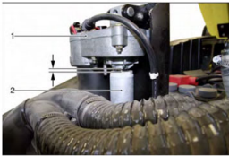
1 Lifting motor 2 Spindles
